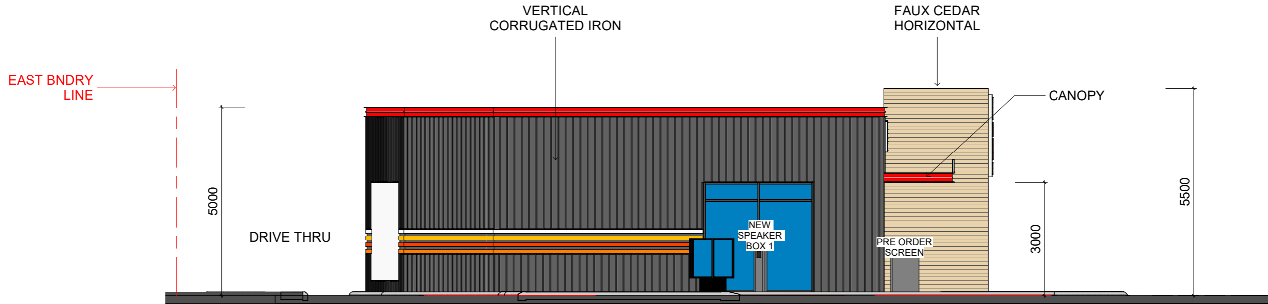
NORTH ELEVATION
