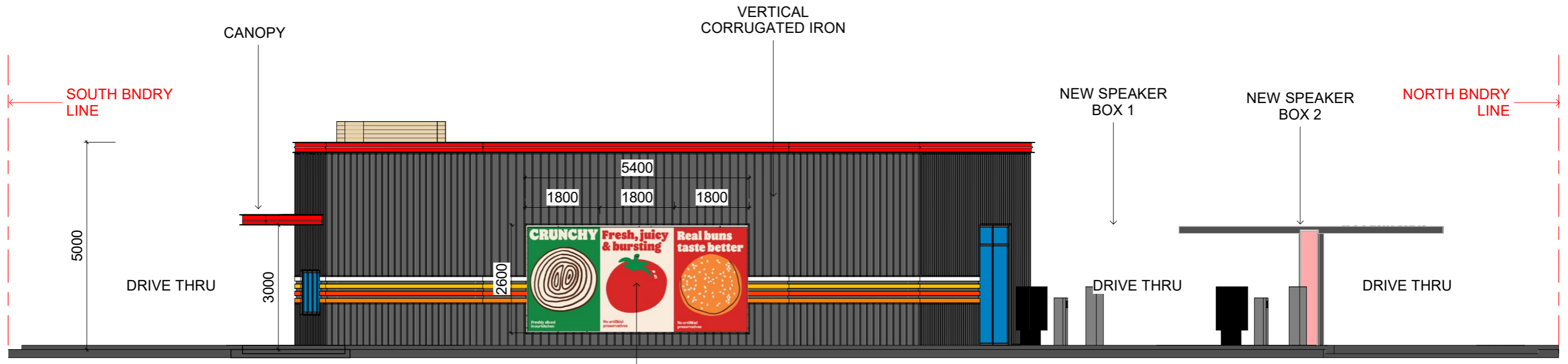
EAST ELEVATION
